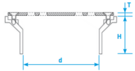
CROSS SECTIONAL VIEW
